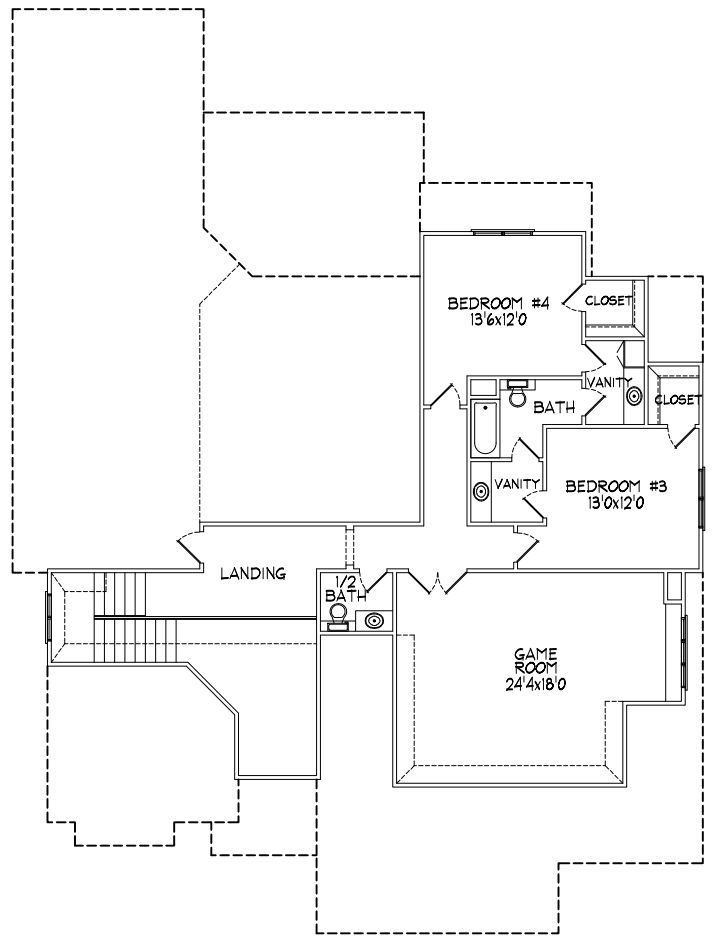
B Upper Level Floor Plan
